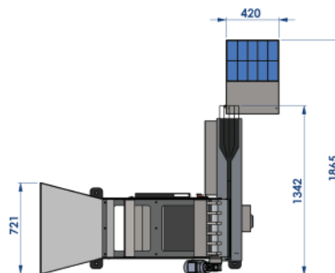
Basic dimensions.
